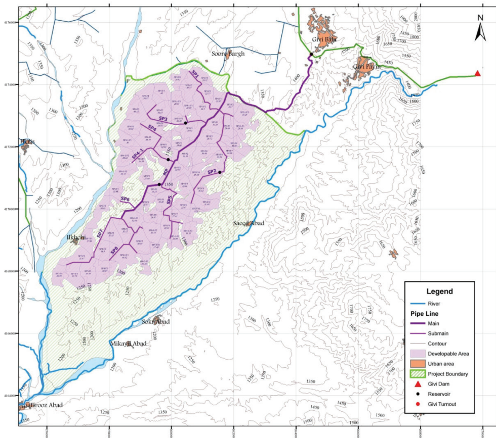
Fig.1. Project layout
