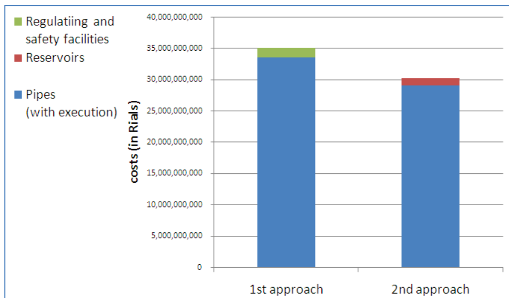
Fig. 3. Cost comparison between the Alternatives A (1st approach) and Alternative B (2nd approach)
