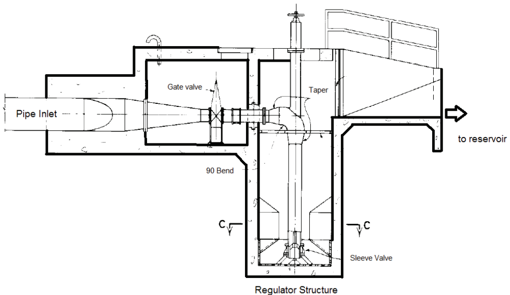
Fig. 2. Regulator Structure (energy dissipater) before reservoirs
