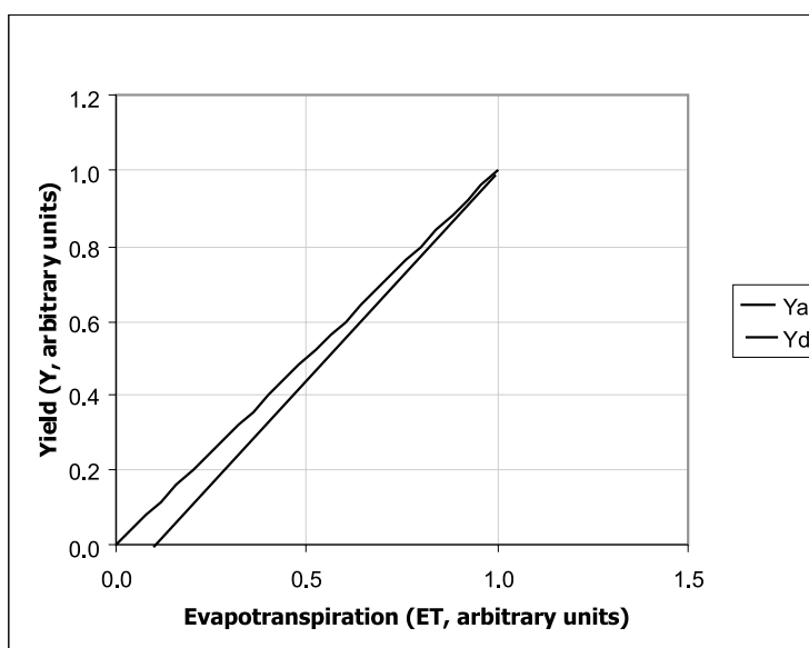
Fig. 1. Theoretical relationships between evapotranspiration and yield from Doorenbos (Ya) and Grismer (Yd). (Relations théoriques entre l'évapotranspiration et le rendement Doorenbos (Ya) et Grismer (Yd)).
